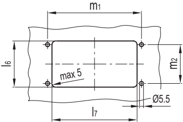
Drilling template
